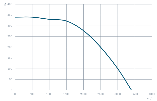
CUB 400
