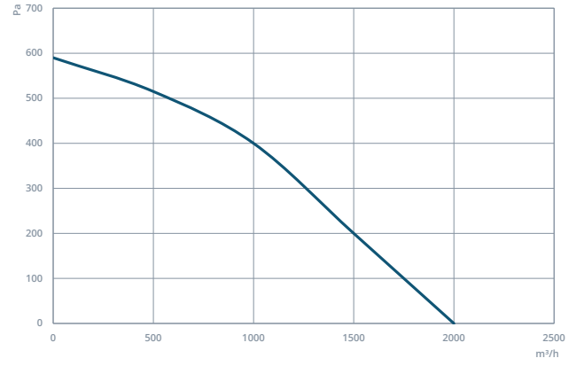
IGK 40
