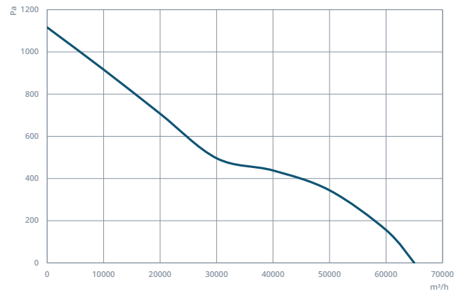
CAXI 1000-8-45
