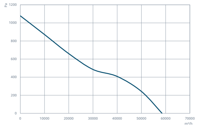
BAXI 1000-8-40
