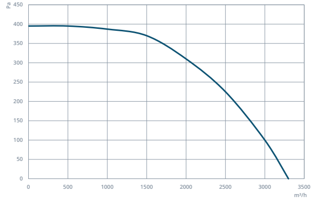
SAL 400
