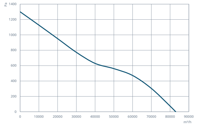
CTAXI 1120-8-40
