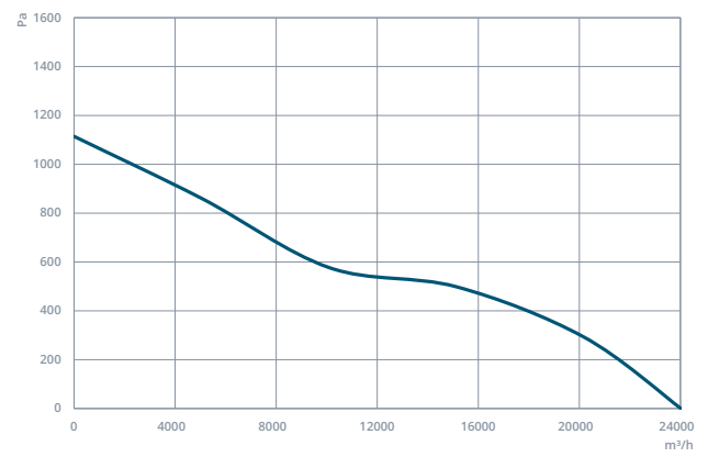
TAXI 560-6-45
